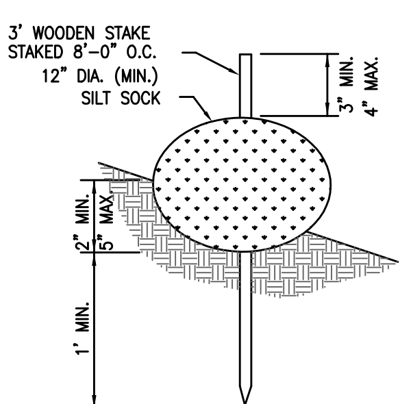
STAKED SILT SOCK DETAIL NOT TO SCALE
