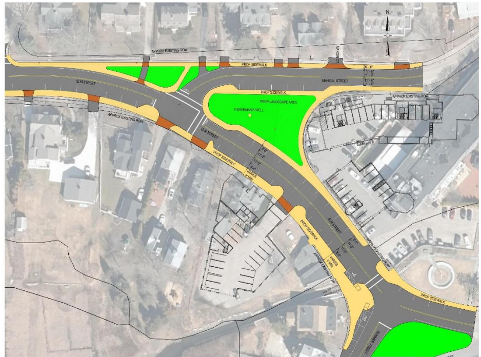
Figure 1: Recommended Reconfigured Intersection at Cohasset Harbor end of Elm St. Corridor
